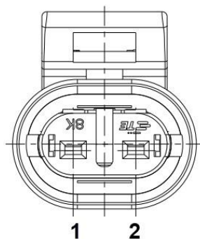
Figure 6: Sensor plug Female, product side view
